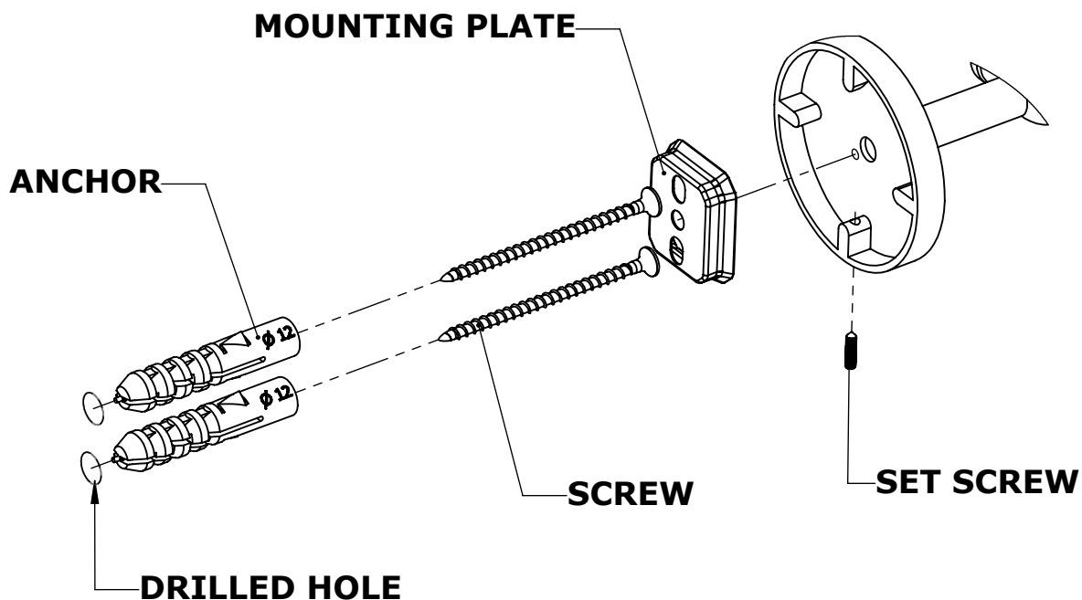
DETAIL M
