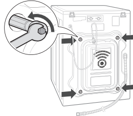
Unpacking and removing shipping bolts
