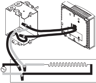
2-wire Installation
