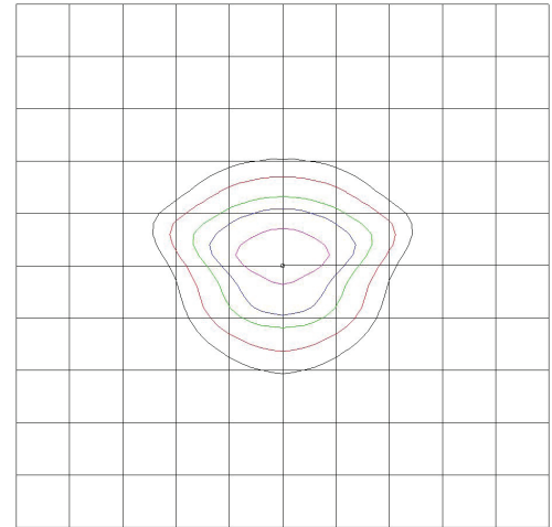
1600 LUMEN CONFIGURATION
