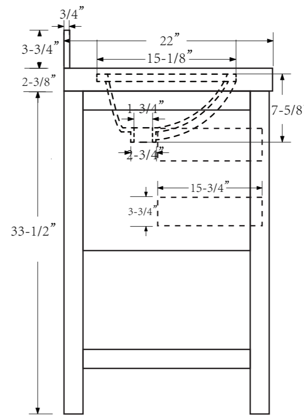
SIDE VIEW
