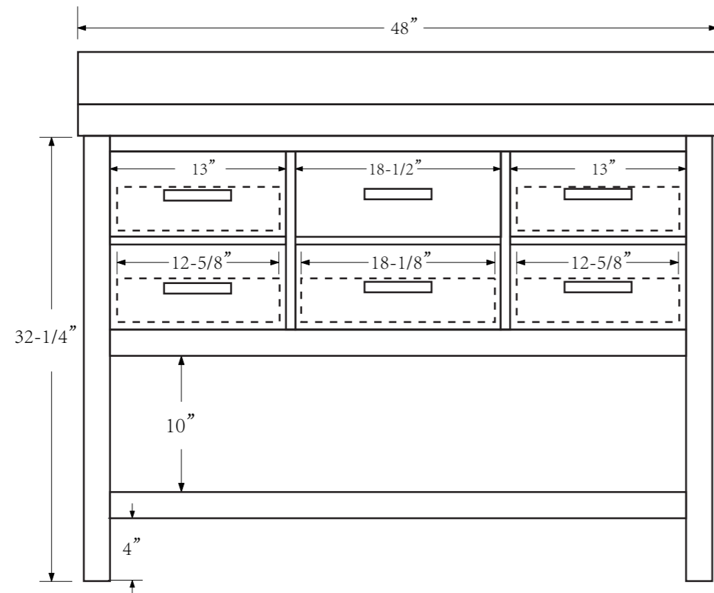
FRONT VIEW
