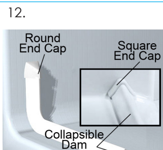
Collapsible Rubber Dam White PVC with End Caps
