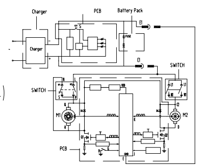
Electric Circuit
