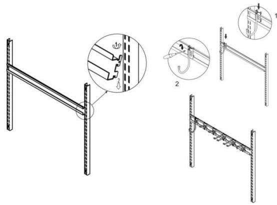
Fig. C-9 – Combination Rail installation
