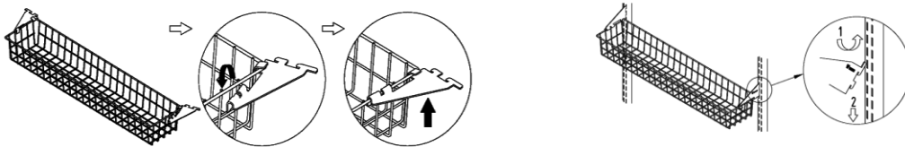
Fig. C-3 Metal Shelf Bracket installation and hanging installation
