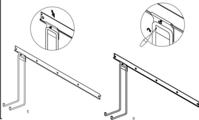
Fig. C-7 – Large Tool Keeper installation
