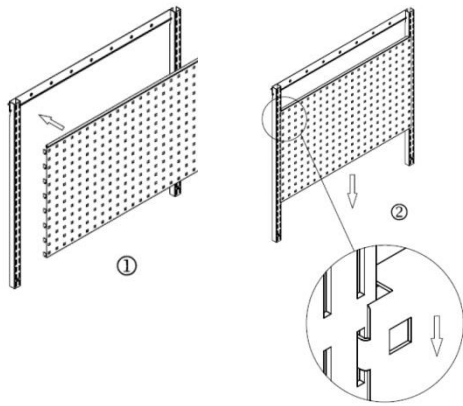
Fig: C-8 – LocBoard installation
