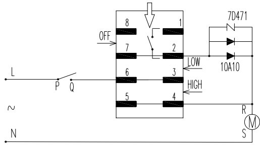
Electric Circuit
