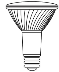
Utilitech-PAR30 Model # PAR30L/5K/LEDG5 15.00W Warm White
