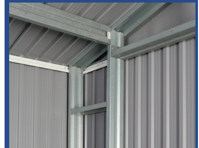
Heavy Reinforced Galvanized Steel Roof Trusses, Beams and wall support
