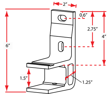
S / L series Wall Bracket
