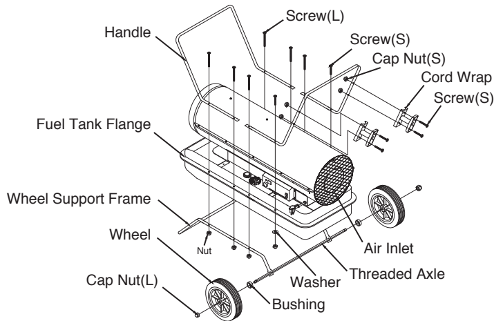
Figure 3. Assembling Handle & Wheel and Cord wrap
