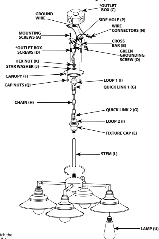
FIGURE 1. For Chandelier Mounting Option
