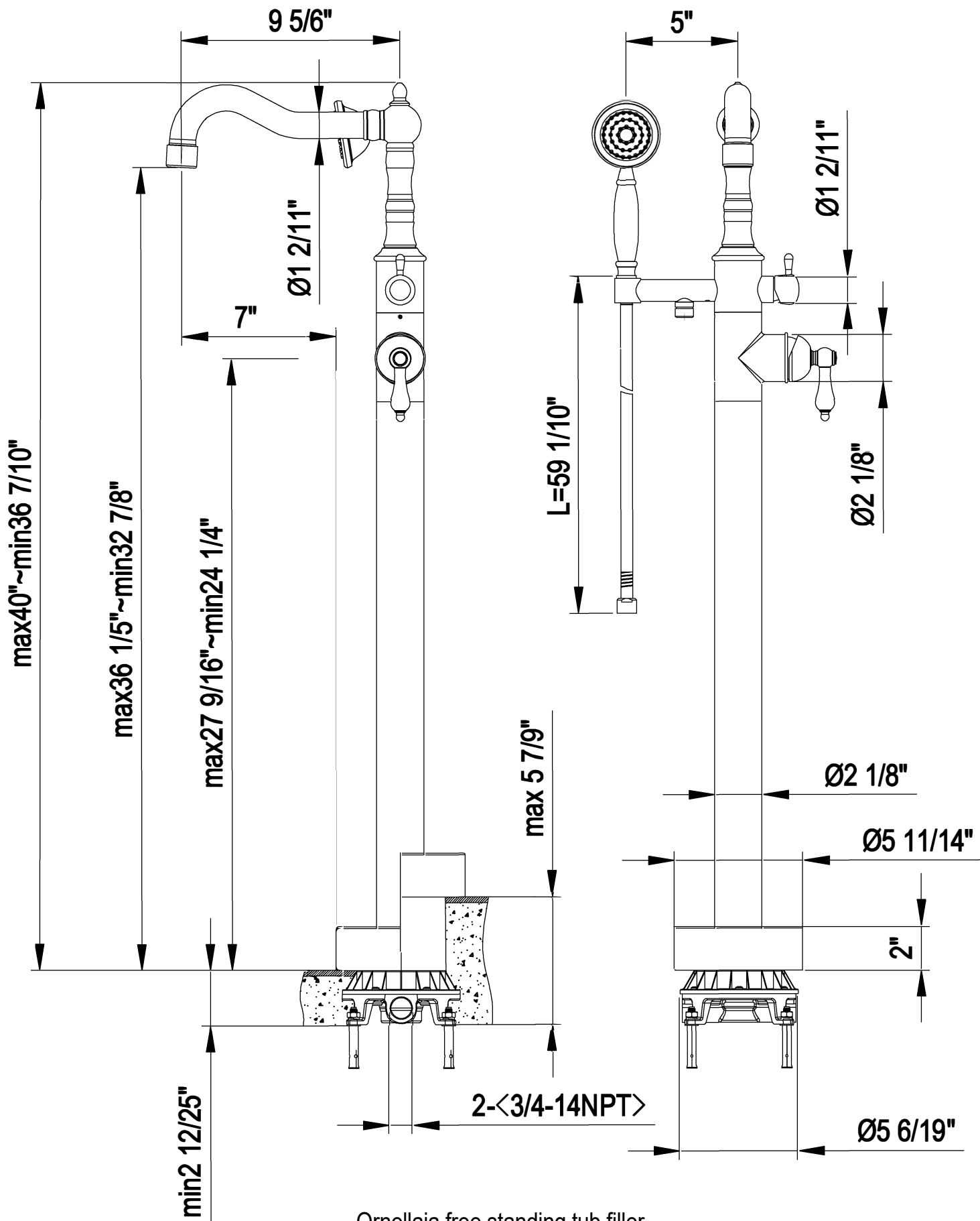
Ornellaia free standing tub filler with hand shower. 12.15 GPM
