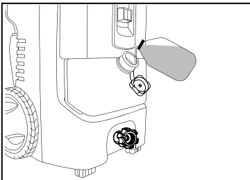
3 Lift up to remove the cap of detergent tank, fill tank with detergent or soap and replace the cap. Apply detergent as instructed by the detergent manufacturer.
