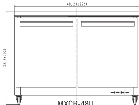
MXCR-48U MXCF-48U
