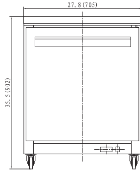
MXCR-27U MXCF-27U
