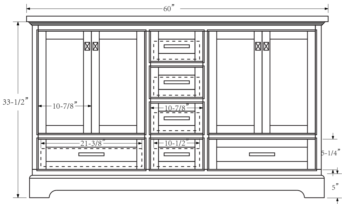
FRONT VIEW
