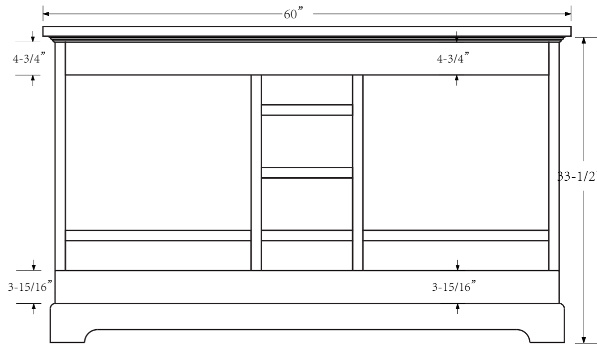
BACK VIEW
