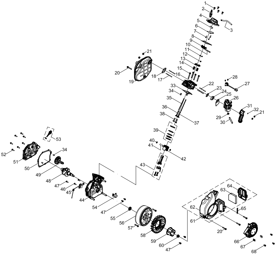
Engine exploded view
