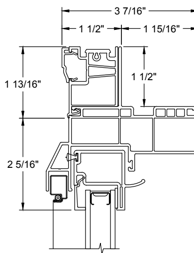
Retro Brickmould
