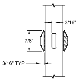
7/8" Contour SDL
