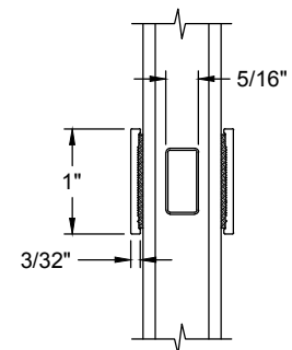
1" Flat SDL
