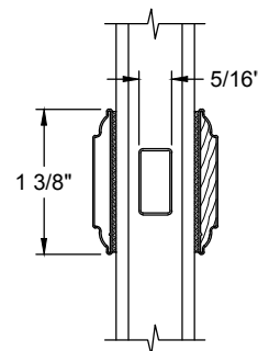
1 3/8" Contour SDL
