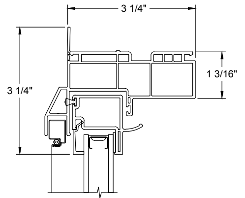
Florida Flange
