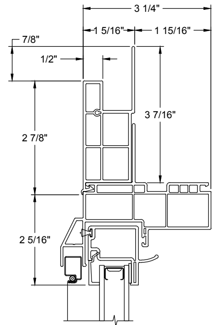
Flat Casing
