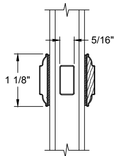
1 1/8" Contour SDL
