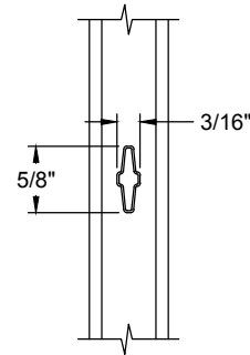
5/8" Contour GBG
