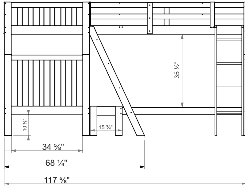
Frontal View
