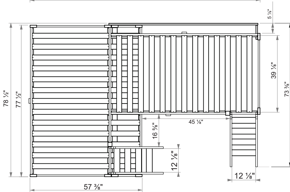
Top View
