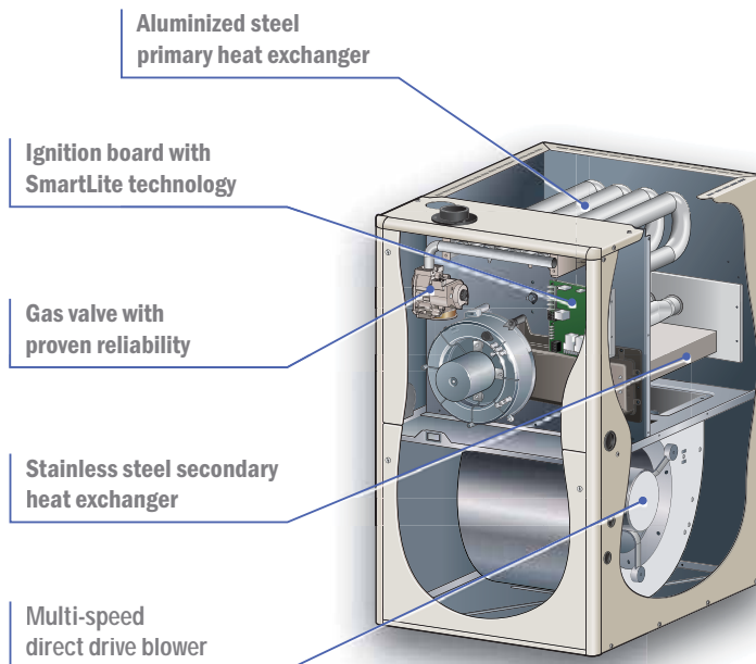
Model MG3P Upflow
