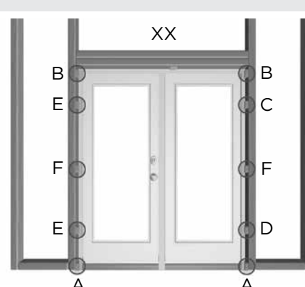
FIGURE 13: Install the shims in the correct locations and in the correct sequence.
