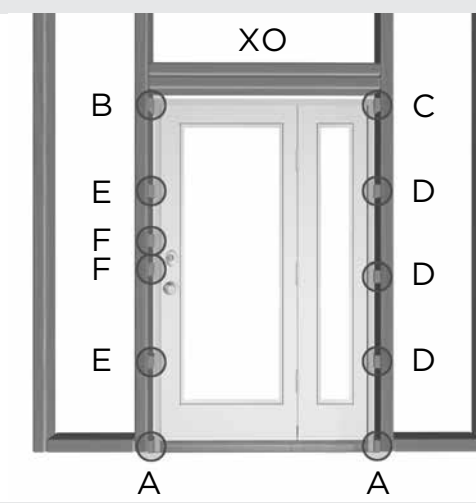
FIGURE 18: Install shims in the correct location and in the correct sequence.
