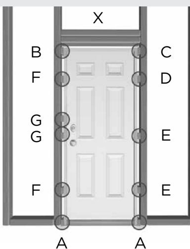
FIGURE 10: Install the shims in the correct locations and in the correct sequence.
