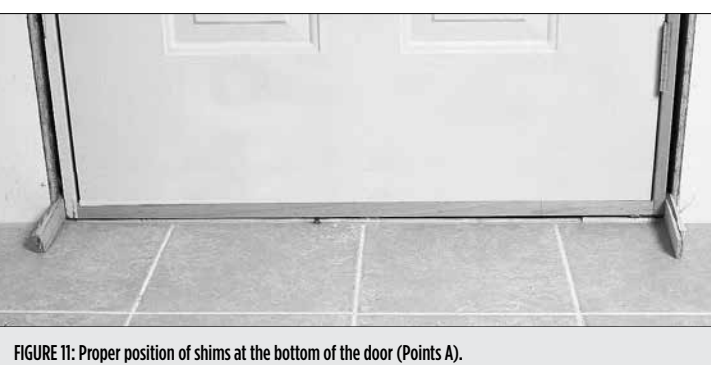
FIGURE 11: Proper position of shims at the bottom of the door (Points A).
