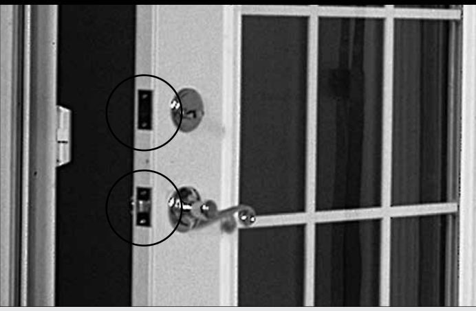
FIGURE 29: The latch and dead bolt are installed per the hardware manufacturer installation detail.
