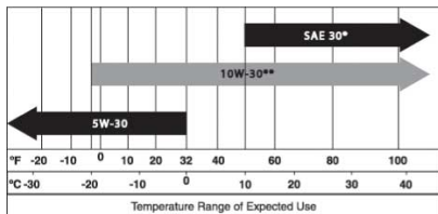
Figure 3-14. Oil Viscosity
