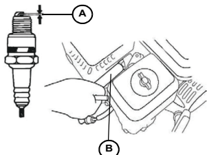
Figure 3-19. Bougie
