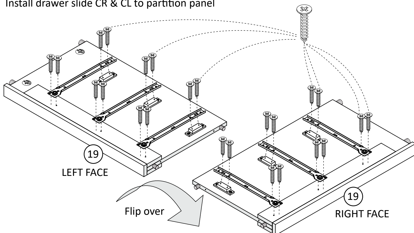
Screw Position on left face
