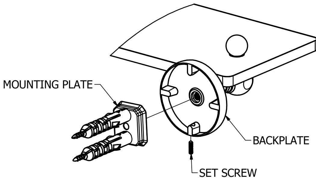
DETAIL D
