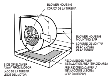
FIGURE 2. SIDEDRAFT COOLER (PARTIAL ILLUSTRATION) FIGURA 2. COOLER DE DESCARGA LATERAL (ILUSTRACION PARCIAL)
