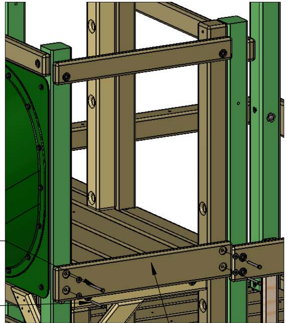
2 X 6 X 30-7/16" SIDE BOTTOM PANEL BOARD
