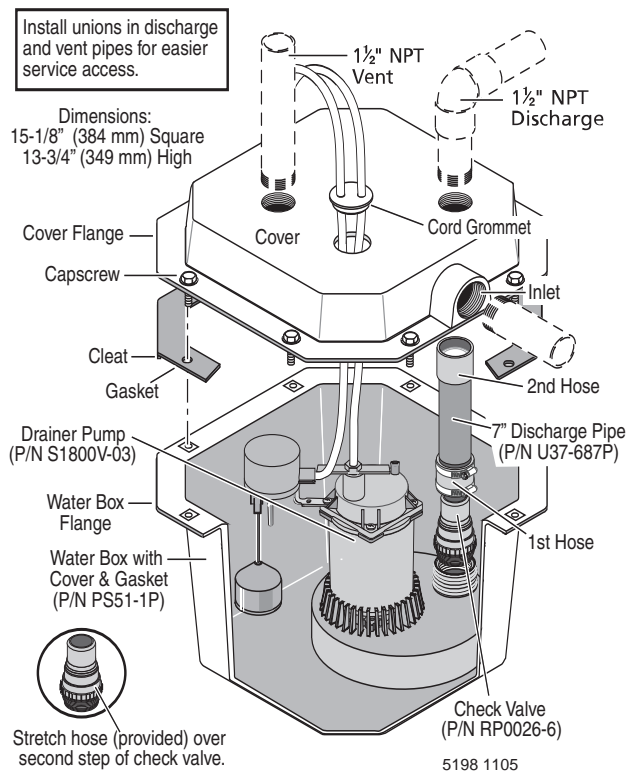
Figure 1 – Laundry Tray Pump System diagram.
