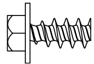
ACV (x6) 5/16" x 5/8" Screw for Plastic
