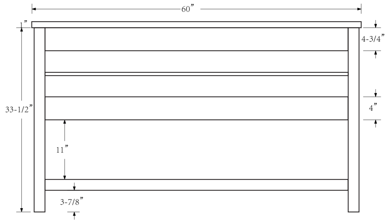
BACK VIEW
