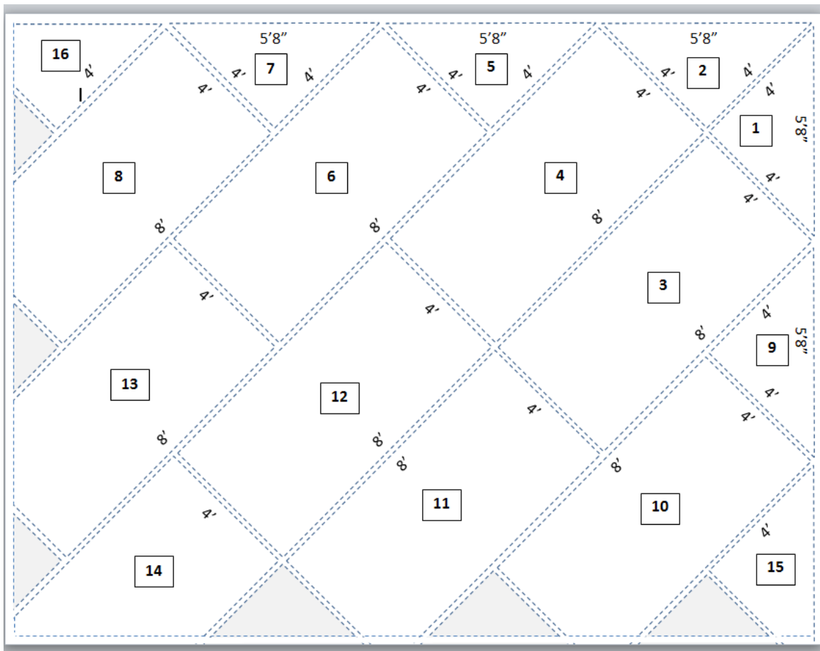
Diagram A - Lay Fiberboard in Diagonal Pattern
