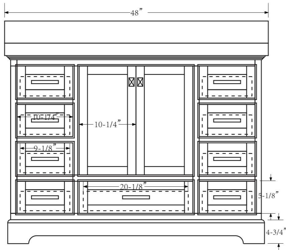
FRONT VIEW
