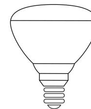
Sylvania-BR30 Model # LED9BR30/DIM /HO/G4/RP 9.00W (2700K)
