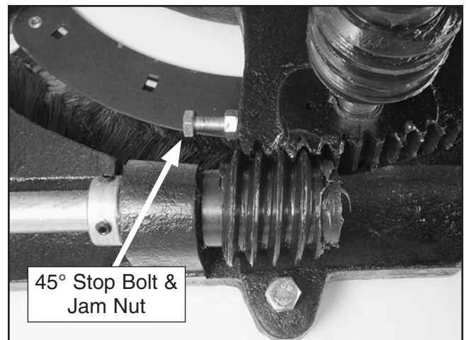
Figure 110. 45° stop bolt and jam nut.
