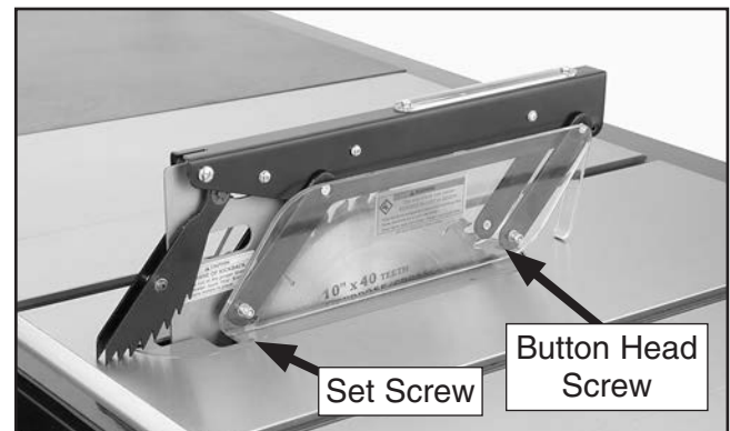
Figure 33. Blade guard installed.
