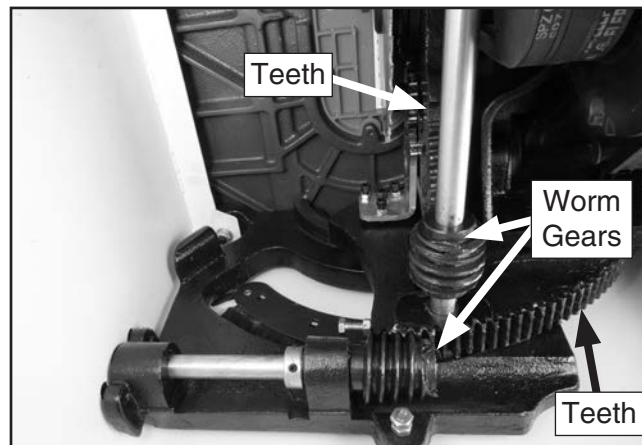
Figure 104. Worm gears and teeth.
