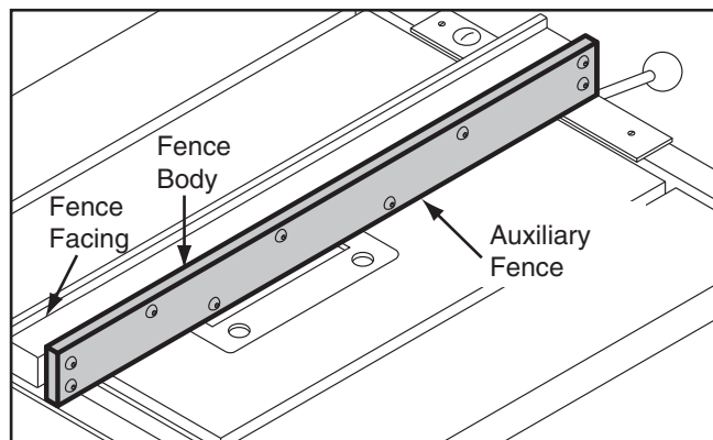
Figure 68. Auxiliary fence.
