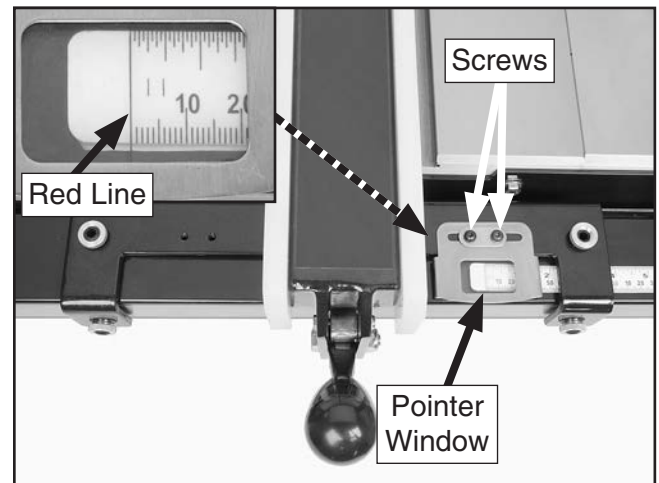
Figure 31. Aligning rail tape with scale pointer.
