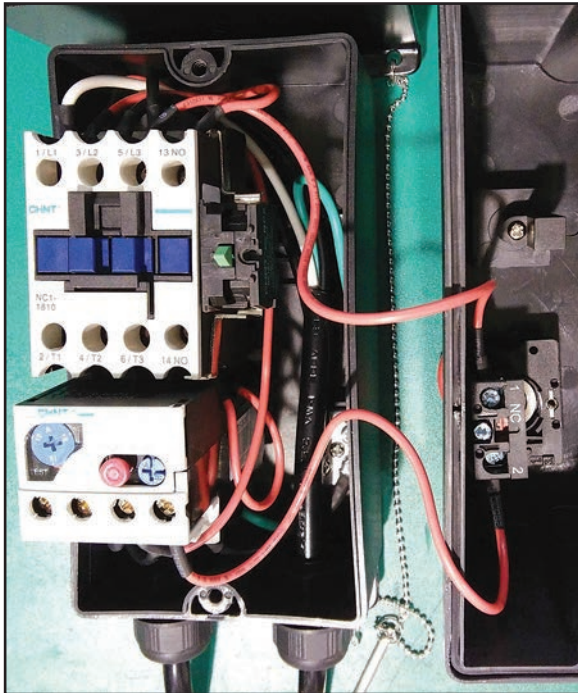
Figure 127. Magnetic switch.
