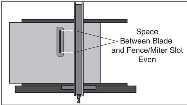
Figure 119. Example of fence aligned parallel to miter slot.
