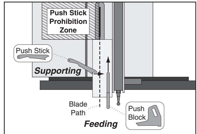
Figure 81. Using a push block and push stick to make a rip cut.
