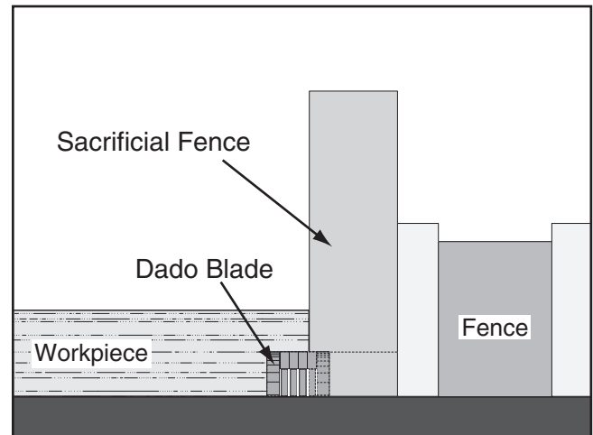
Figure 64. Rabbet cutting.
