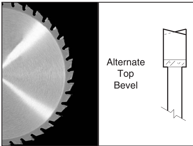
Figure 44. Crosscutting blade.
