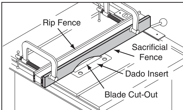
Figure 63. Sacrificial fence.
