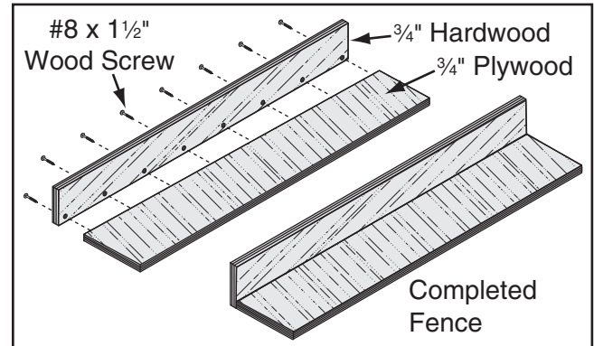
Figure 84. Location of pilot holes.
