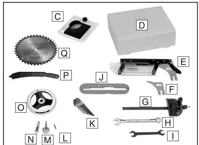
Figure 5. Component inventory.
