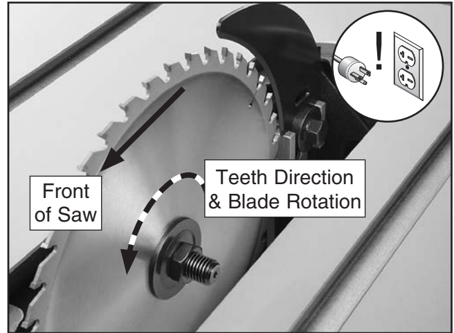
Figure 48. Example of correct blade direction.
