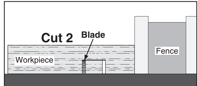
Figure 61. Second cut for a single blade dado.
