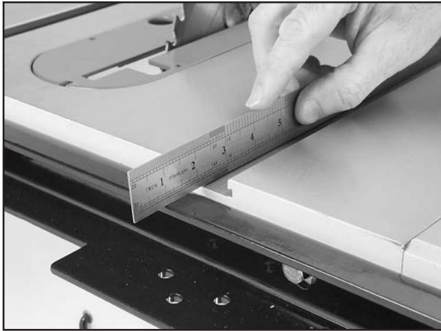
Figure 22. Verifying rear rail is flush with bottom of T-slot.
