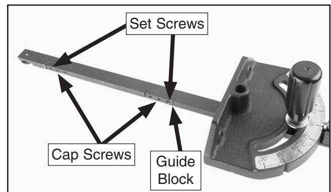
Figure 124. Screws for adjusting miter bar in miter slot.
