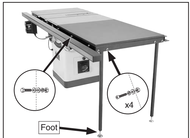
Figure 25. Model G0691 extension table installed.
