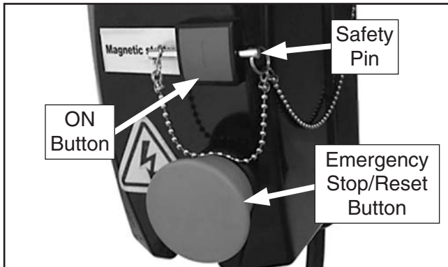
Figure 39. Power controls.
