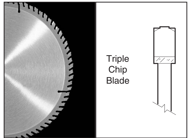
Figure 46. Laminate blade.
