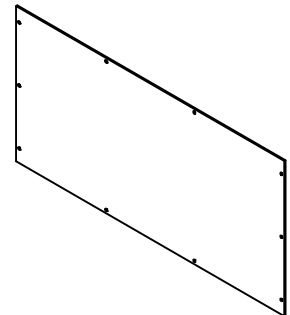
BACK PANEL QTY 1
