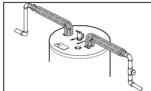
Typical Horizontal piping arrangement.
