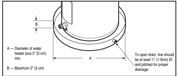
Figure 1. — Auxiliary Catch Pan
