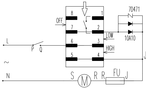
Electric Circuit
