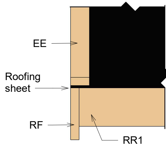
3 Roof Reinforcement
