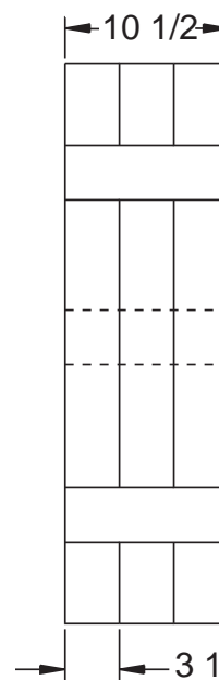
3 Wide Board-N-Batten Joined Assembly
