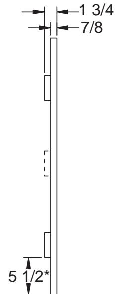
3 Wide Board-N-Batten Joined Assembly
