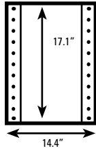
PLATFORM DIMENSIONS (INCLUDES STEP)
