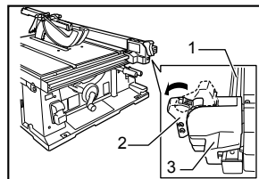
1. Guide rail 2. Knob 3. Hook
