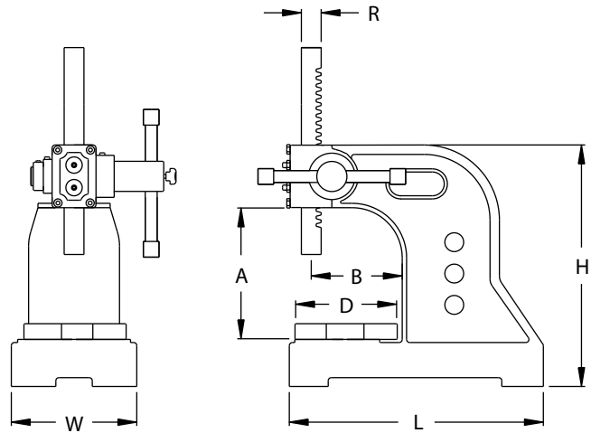
Figure 1 - Dimensions
