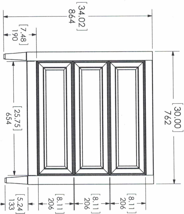
Front View
