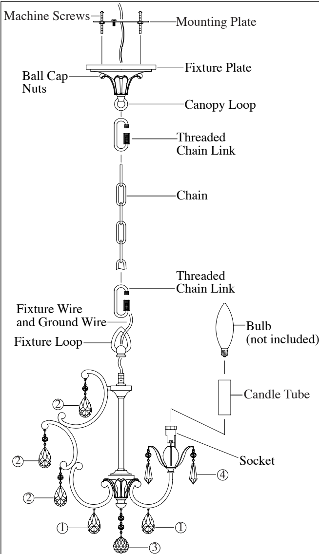
FIG: 1 CHAIN HUNG INSTALLATION
