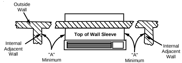
Figure 2 - Minimum Wall Opening Dimensions
