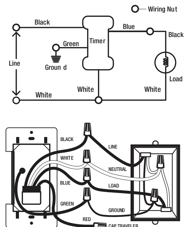
Figure 2 - Typical Wiring Schematic for Single Pole Installation
