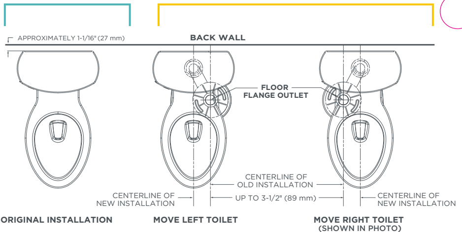
AccessPRO saves both time and money relocating toilet toward or away from the secondary wall (no floor flange outlet change required)
