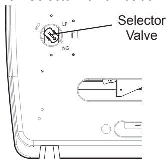
Fig. 4a - Selector Valve Positioning
