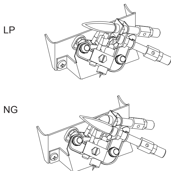
Fig. 26 - Correct Pilot Flame Pattern
