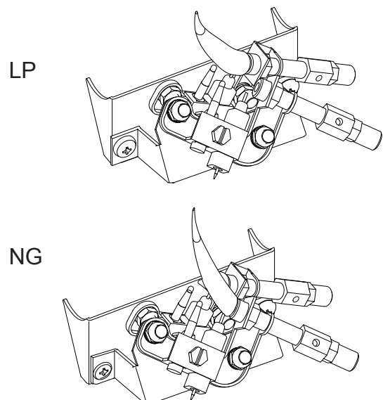
Fig. 27 - Incorrect Pilot Flame Pattern
