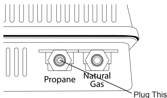
Fig. 5a - Regulator Plug Location
