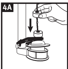
4A FOR GLACIER BAY TOILETS: PUSH FLOAT DOWN TO FLAPPER FRAME.
